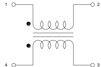
EQUIVALENT CIRCUIT
